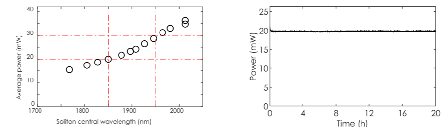
Evolution of the soliton average power vs the soliton central wavelength and brun-in on 20 hours @1900 nm.
